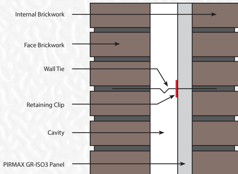
Double Brick Cavity Wall Side Elevation
